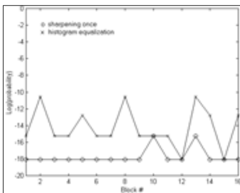
Figure 6. Robustness to sharpening and histogram equalization.
