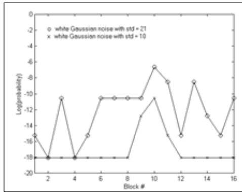
Figure 4. Robustness to white Gaussian noise.
