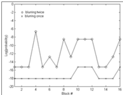
Figure 5. Robustness to repeated blurring.
