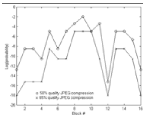
Figure 7. Robustness to JPEG compression.
