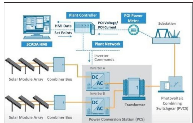
Figure 2. Photovoltaic System Architecture 2 describes Photovoltaic System Architecture.
